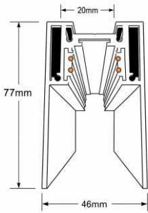
PRODUCT DIMENSION
