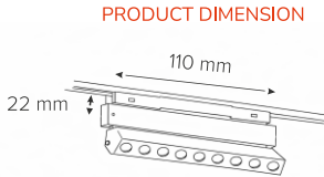
PRODUCT DIMENSION
