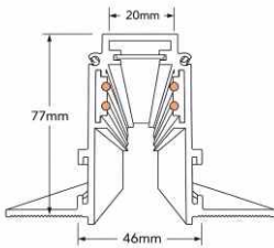
PRODUCT DIMENSION
