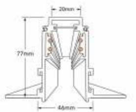
PRODUCT DIMENSION
