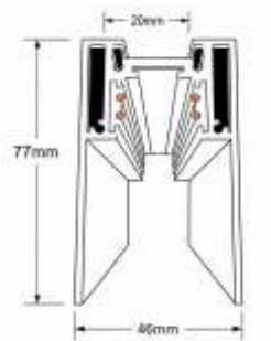
PRODUCT DIMENSION
